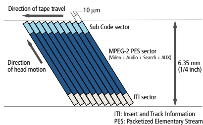
Track Pattern of the HDV 1080i Specification
